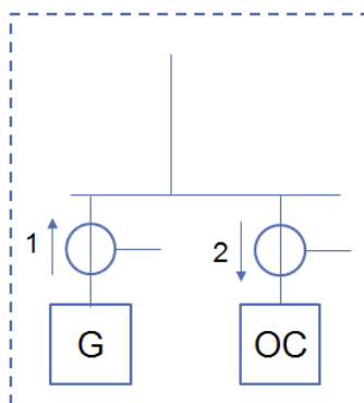
Figure 9. Gross metering of production.
